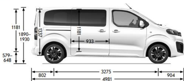
Zafira Electric Alle Maße in mm
