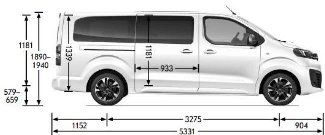
Zafira Electric XL Alle Maße in mm
